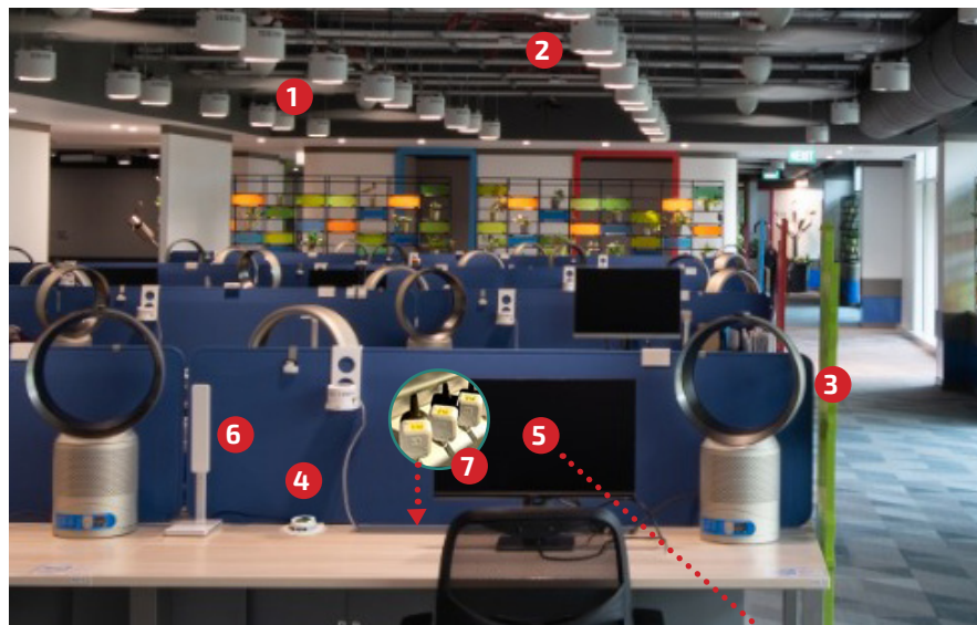
Closed-loop control over PoE lighting and roller blinds utilizing desktop sensor maximizing daylight while providing individual task lighting.
